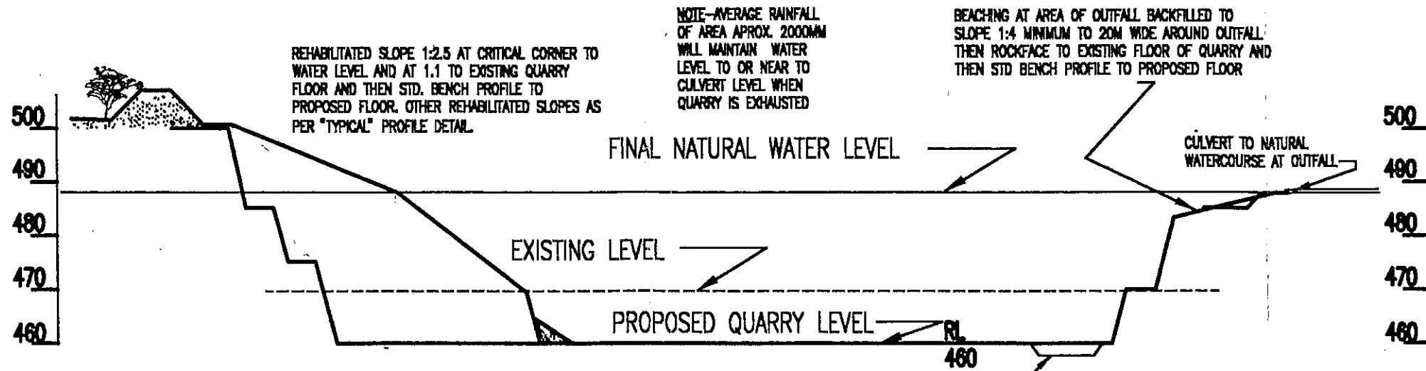
REHABILITATION SECTION "DD" 1:1000
