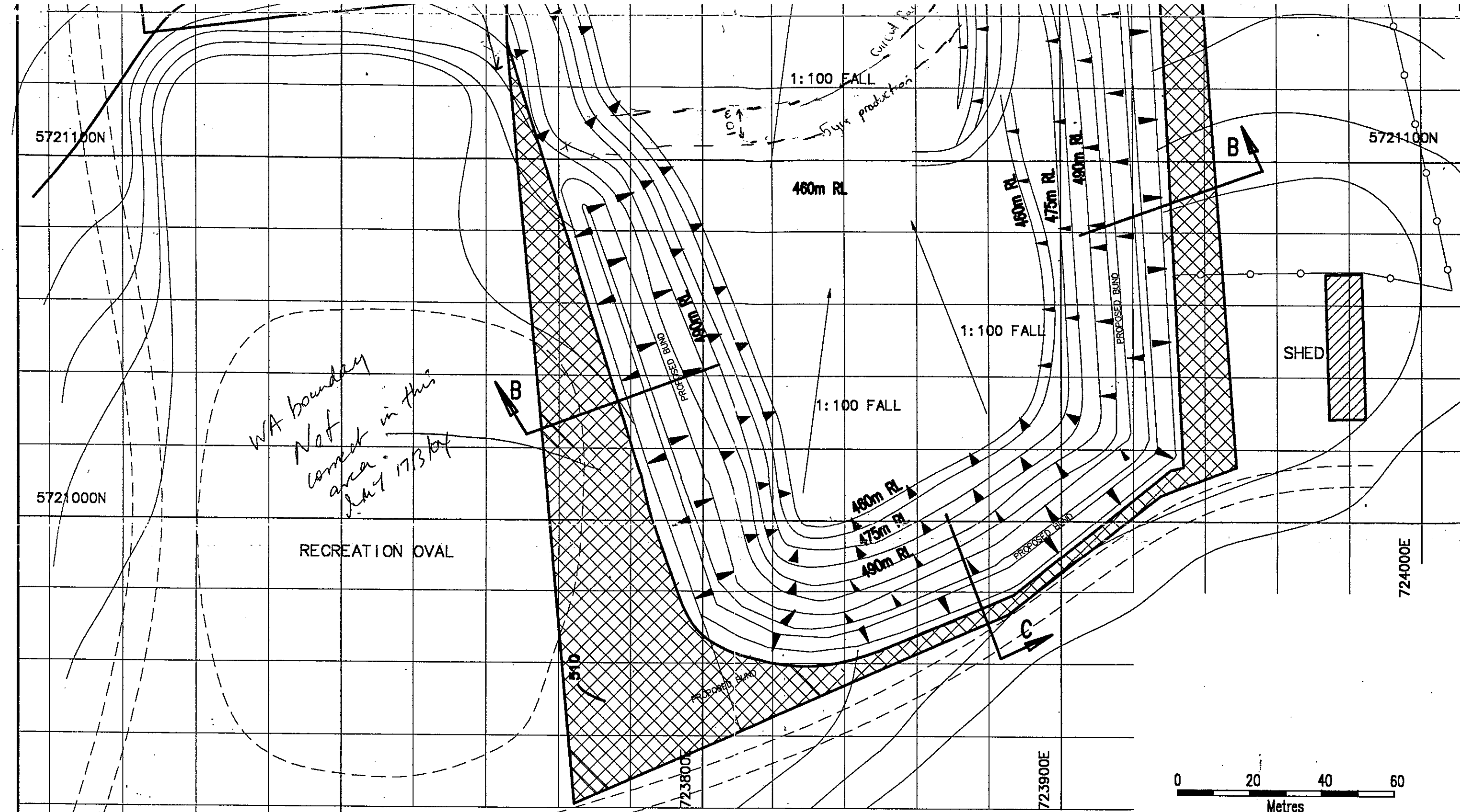
PROPOSED AMENDED EXTENT OF EXTRACTION 1:1000
