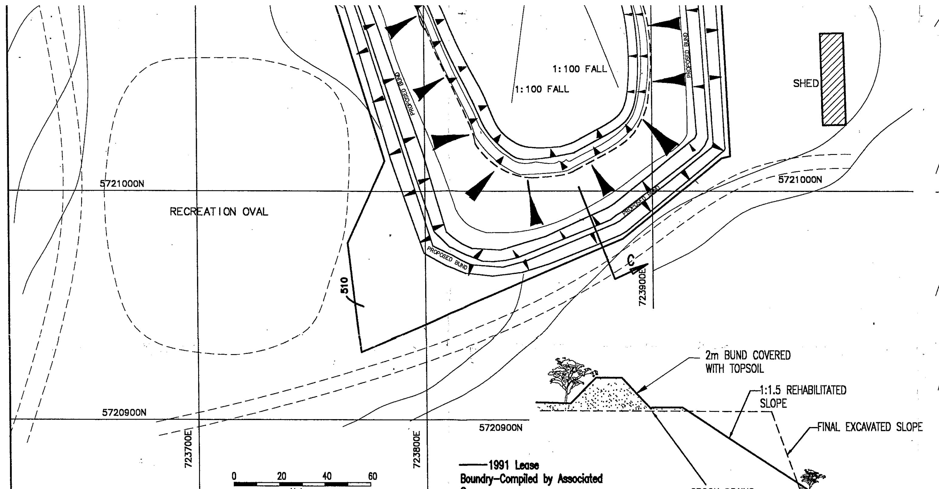
TYPICAL REHABILITATION SLOPE SCALE 1:500
